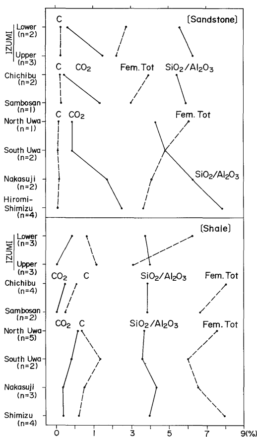
Fig. 3 Time-space variation of selected chemical components, as shown by average values of individual sedimentary units. Fem. Tot. implies sum of \text{TiO}_2 , \text{Fe}_2\text{O}_3 , \text{FeO} , \text{MnO} and \text{MgO} .
