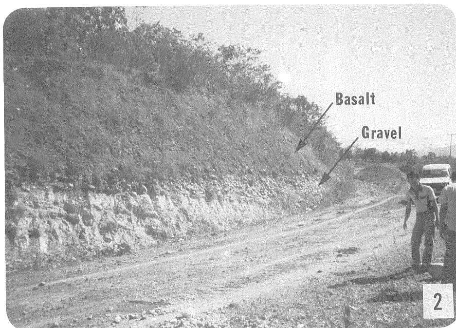
2 Outcrop of basalt (sample 82Z0402) overlying the gravel deposit in the southern Mae Moh Basin.
