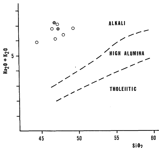
Fig. 4 Total alkalis, plotted against SiO 2 for the Lampang basalt. Open circles are present data, and solid circles are the data from BARR and MACDONALD (1978, 1981). Dashed lines represent boundaries of Japanese basalt types (KUNO, 1966).
