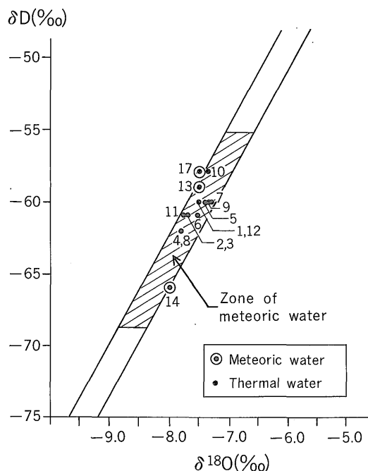
Fig. 3 Diagram of \delta D - \delta^{18}O of waters from the San Kamphaeng area.
