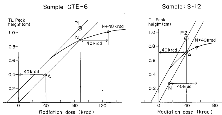
Fig. 6 Graphical correction of TL Saturation. A : Artificially irradiated sample N : Natural sample P1 : Saturation corrected TL peak height for natural sample P2 : Saturation corrected TL peak height for Artificially irradiated sample
