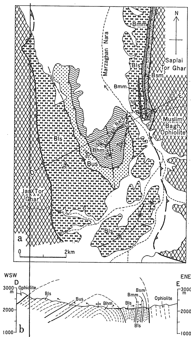
Fig. 4 Geologic map of the Bagh Complex in the western part of the Muslim Bagh area. Legends are the same with those of Fig. 3.
