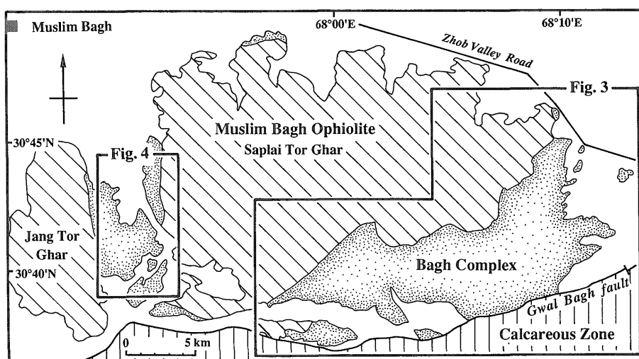
Fig. 2 Map showing the lithologic subdivision of the Muslim Bagh area in Pakistan, and also showing the areas of Figs. 3 and 4.
