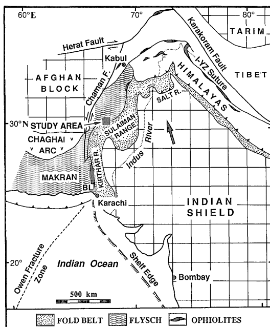
Fig. 1 Tectonic map in and around Pakistan (simplified from Humayon et al. , 1991). Black square shows the study area (Muslim Bagh area), and the big arrow indicates direction of the general convergence of the Indian subcontinent relative to Asia. Cross stripes indicate the Indian shield and microcontinents. I-YZ Suture: Indus Yarlung-Zangbo suture, BL: Bela Ophiolite.
