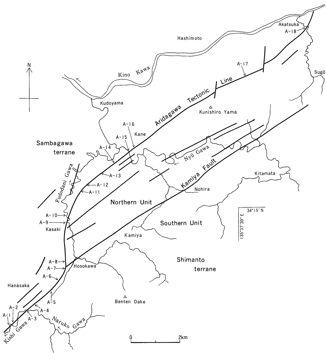
Fig. 6 Aridagawa Tectonic Line and subsidiary faults in the Kudoyama area, Wakayama Prefecture.
