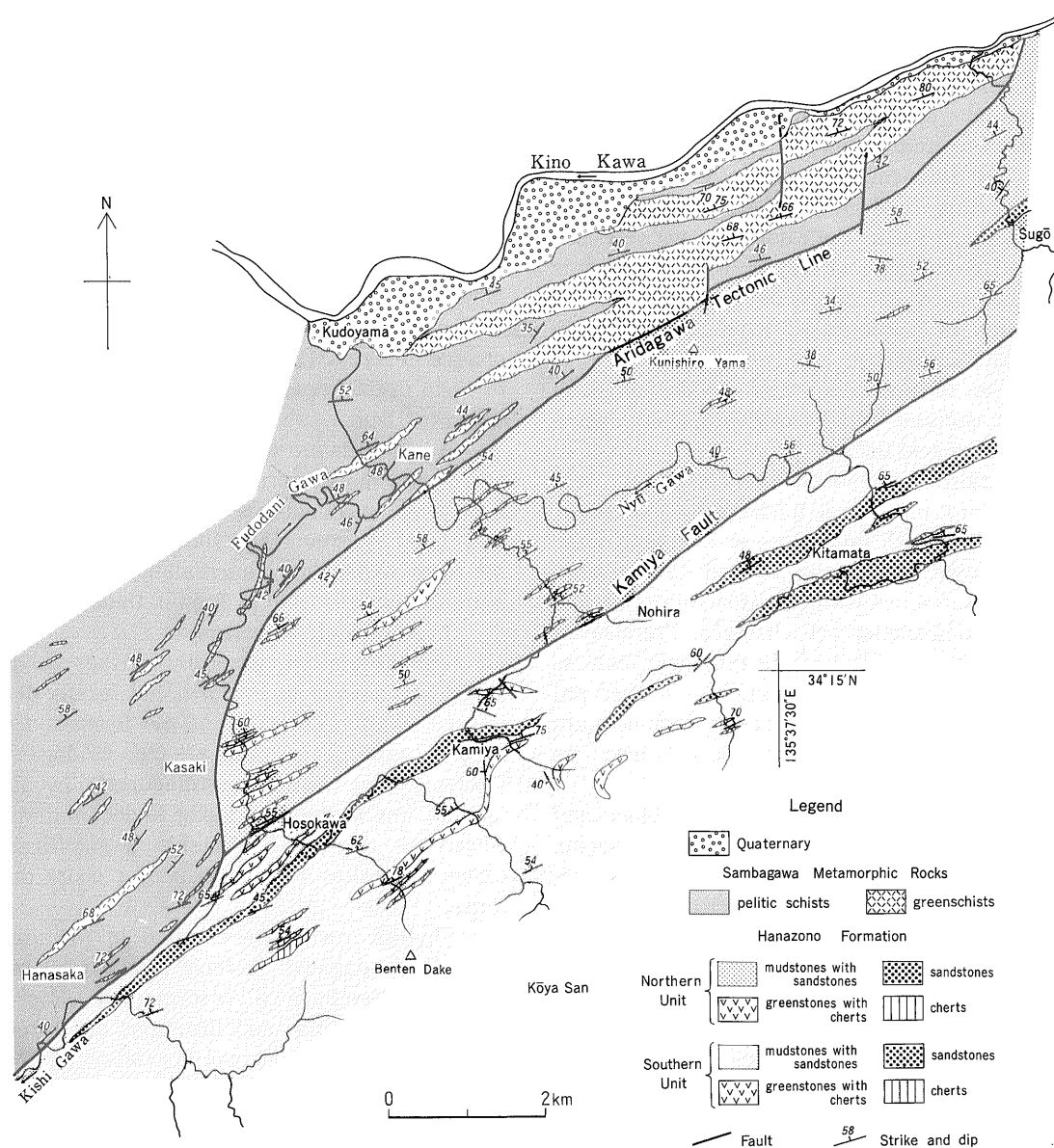
Fig. 3 Geological map of the Kudoyama area.
