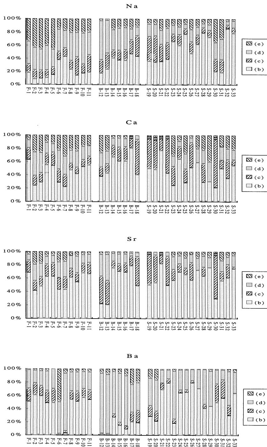
Fig. 6 Percentages among fractions of diagenetic processes. : (b) AcONH 4 soluble fraction ; (c) AcOH soluble fraction ; (d) NH 2 OH · HCl soluble fraction ; (e) H 2 O 2 soluble fraction. F-1 to F-11, B-12 to B-18 and S-19 to S-33 are fresh-water lake samples, brackish-water lake samples and sea samples, respectively.
