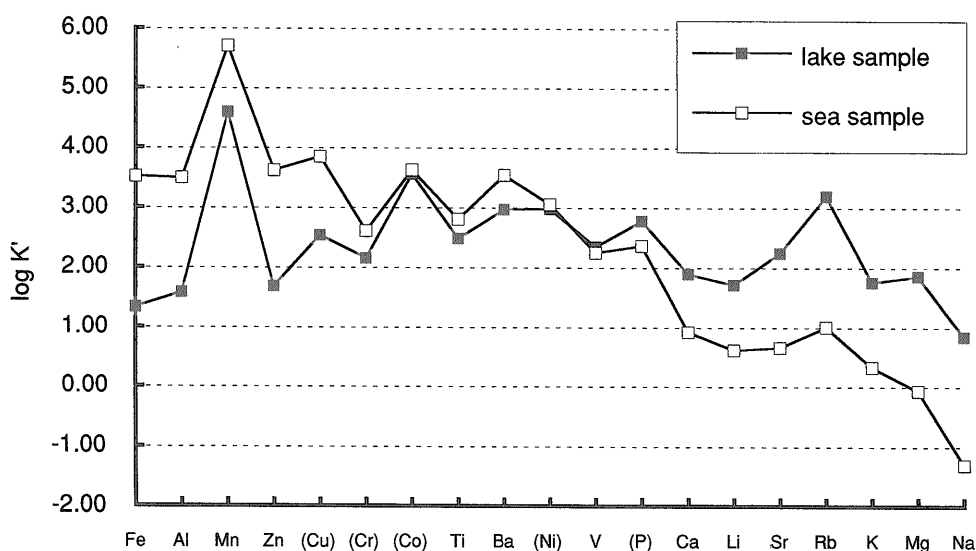
Fig. 8 Variation of ion exchange constant ( K' ) calculated from \text{AcONH}_4 soluble fraction. Elements in the parentheses are shown for reference.
