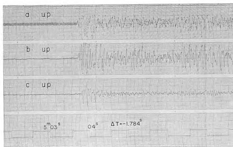
Fig. 5-8 Seismograms obtained (22) at D_6 , (23) at D_7 and (24) at D_8 from the shot A-II
