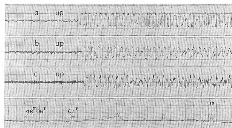
Fig. 5-46 Seismograms obtained (136) at D_7 , (137) at D_8 and (138) at D_9 from the shot B-I
