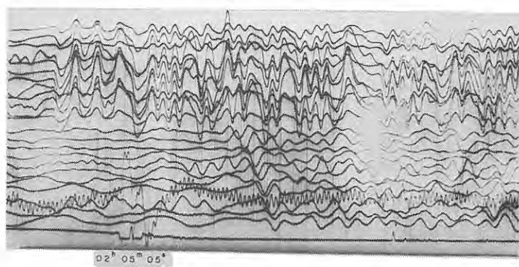
Fig. 6-1 Seismograms obtained (1) at E_1 , (2) at E_2 and (3) at E_3 from the shot A-I
