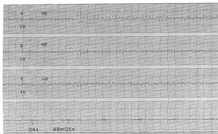
Fig. 5-54 Seismograms obtained (160) at D_1 , (161) at D_2 and (162) at D_4 from the shot B-III 1
