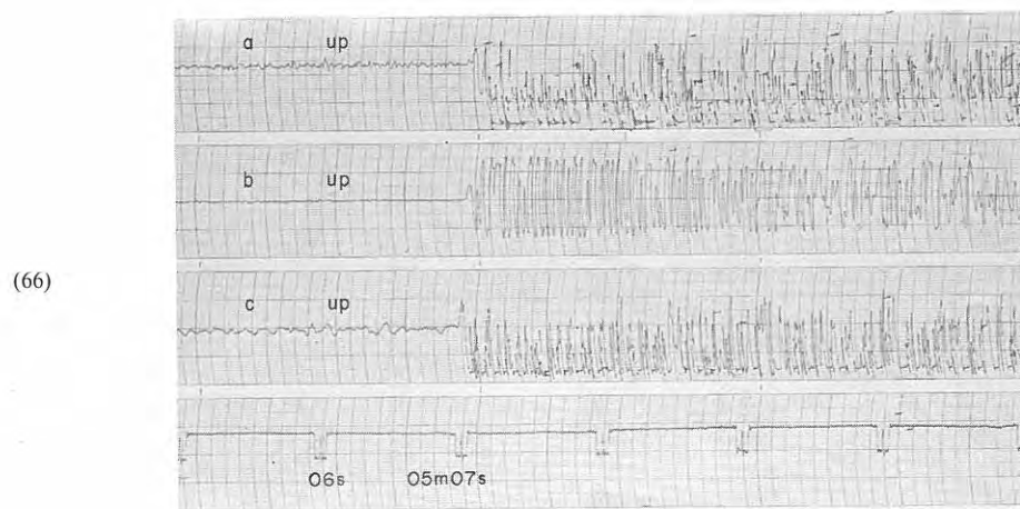
Fig. 5-22 Seismograms obtained (64) at D_{14} from the shot A-IV 1 , and (65) at D_1 and (66) at D_2 from the shot A-IV 2
