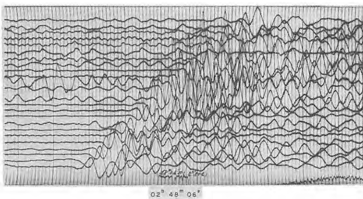
Fig. 6-20 Seismograms obtained (58) at E_5 from the shot B-III 2 , and (59) at E_1 and (60) at E_2 from the shot B-IV
