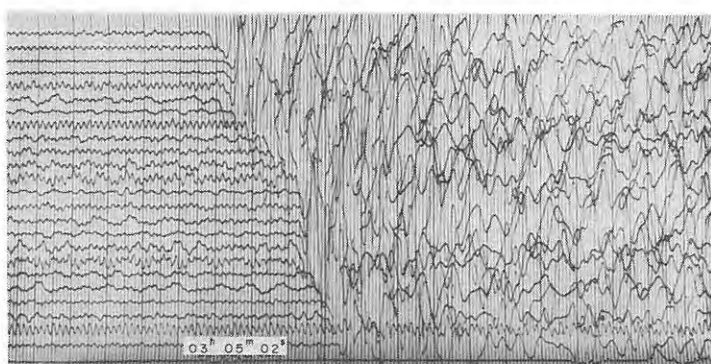
Fig. 6-5 Seismograms obtained (13) at E_3 , (14) at E_4 and (15) at E_5 from the shot A-III
