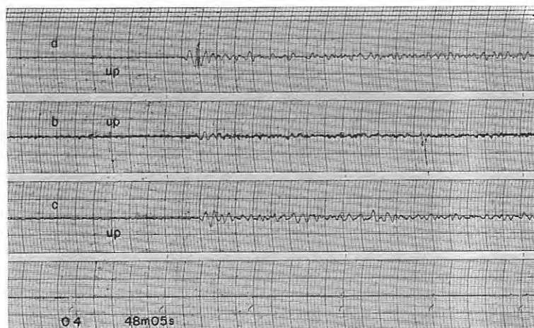
Fig. 5-52 Seismograms obtained (154) at D_{10} , (155) at D_{11} and (156) at D_{12} from the shot B-II
