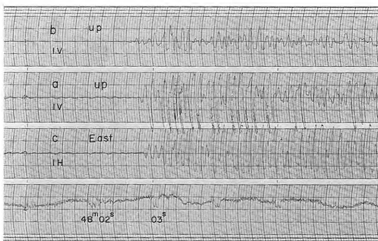
Fig. 5-44 Seismograms obtained (130) at D 1 , (131) at D 2 and (132) at D 3 from the shot B-I
