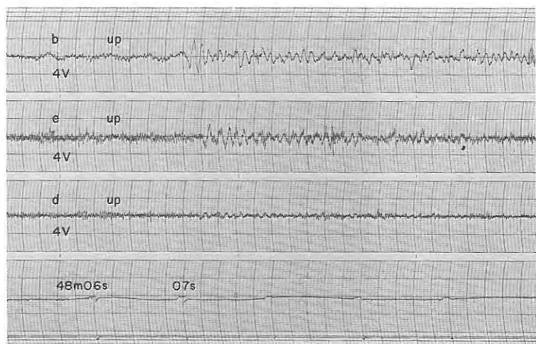
Fig. 5-53 Seismograms obtained (157) at D_{13} , (158), (159) at D_{14} from the shot B-II
