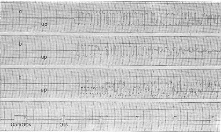
Fig. 5-25 Seismograms obtained (73) at D_8' , (74) at D_9 and (75) at D_{10} from the shot A-IV 2
