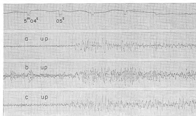
Fig. 5-11 Seismograms obtained (31), (32) at D_{14} from the shot A-II, and (33) at D_1 from the shot A-III
