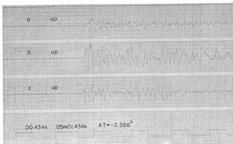
Fig. 5-24 Seismograms obtained (70) at D_6 , (71) at D_7 and (72) at D_8 from the shot A-IV 2
