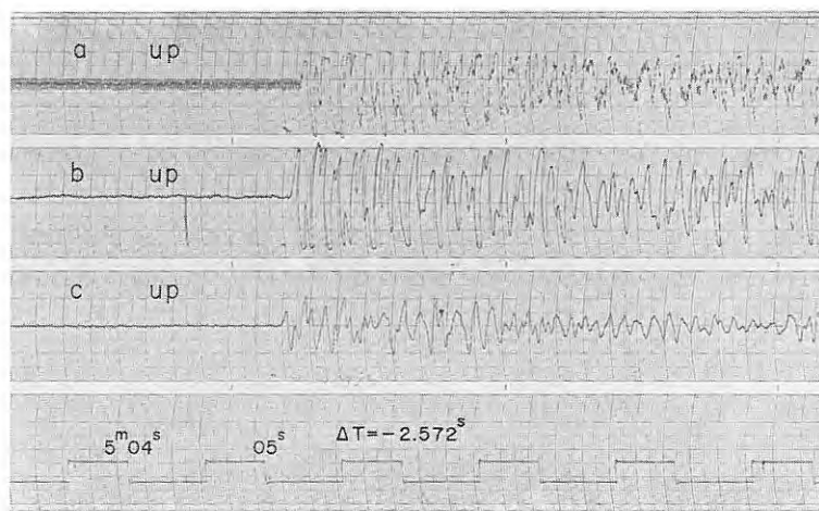
Fig. 5-35 Seismograms obtained (103) at D_6 , (104) at D_7 and (105) at D_8 from the shot A- V_2
