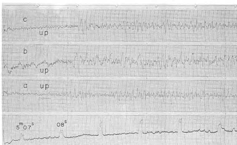
Fig. 5-10 Seismograms obtained (28) at D_{11} , (29) at D_{12} and (30) at D_{13} from the shot A-II
