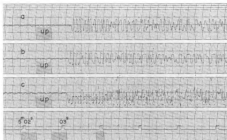
Fig. 5-36 Seismograms obtained (106) at D_8' , (107) at D_9 and (108) at D_{10} from the shot A-V 2
