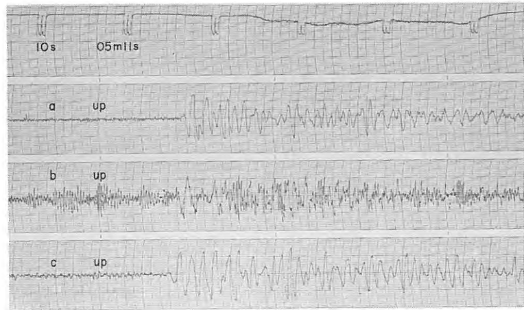
Fig. 5-27 Seismograms obtained (79), (80) at D_{14} from the shot A-IV 2 , and (81) at D_1 from the shot A-V 1
