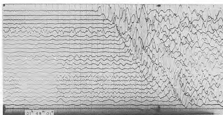
Fig. 6-15 Seismograms obtained (43) at E_4 and (44) at E_5 from the shot B-I, and (45) at E_1 from the shot B-II
