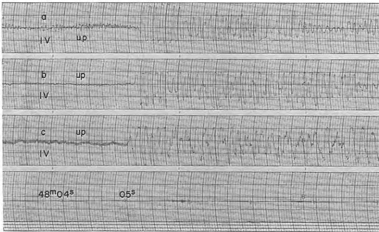
Fig. 5-59 Seismograms obtained (175) at D 2 , (176) at D 3 and (177) at D 4 from the shot B-III 2
