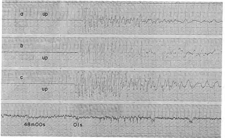
Fig. 5-55 Seismograms obtained (163) at D 5 , (164) at D 6 and (165) at D 7 from the shot B-III 1
