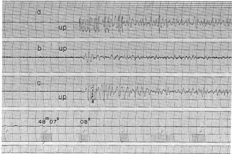
Fig. 5-47 Seismograms obtained (139) at D_{10} , (140) at D_{11} and (141) at D_{12} from the shot B-I
