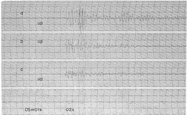
Fig. 5-31 Seismograms obtained (91) at D_{10} , (92) at D_{11} and (93) at D_{12} from the shot A- V_1
