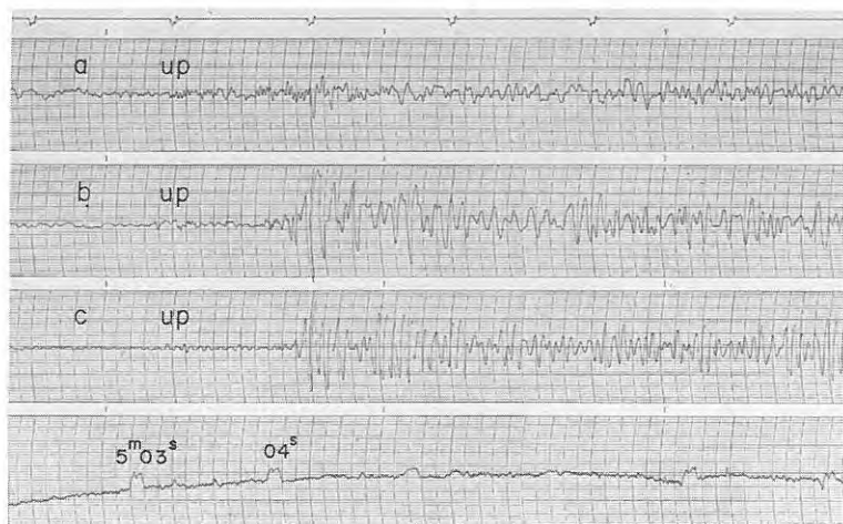
Fig. 5-41 Seismograms obtained (121) at D_8 , (122) at D_8' and (123) at D_9 of profile A from the shot B-IV
