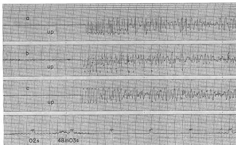
Fig. 5-66 Seismograms obtained (196) at D_8 , (197) at D_9 and (198) at D_{10} from the shot B-IV
