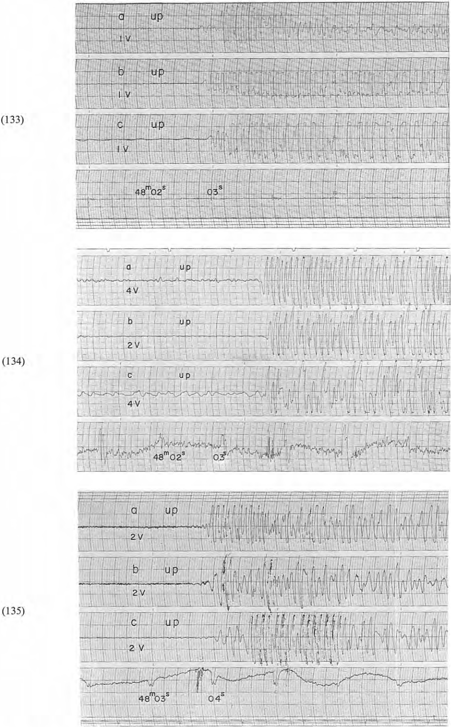
Fig. 5-45 Seismograms obtained (133) at D 4 , (134) at D 5 and (135) at D 6 from the shot B-I
