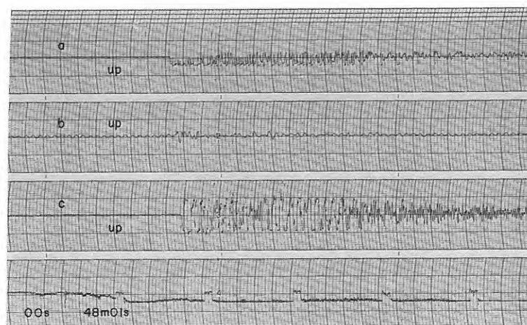
Fig. 5-56 Seismograms obtained (166) at D_8 , (167) at D_9 and (168) at D_{10} from the shot B-III 1
