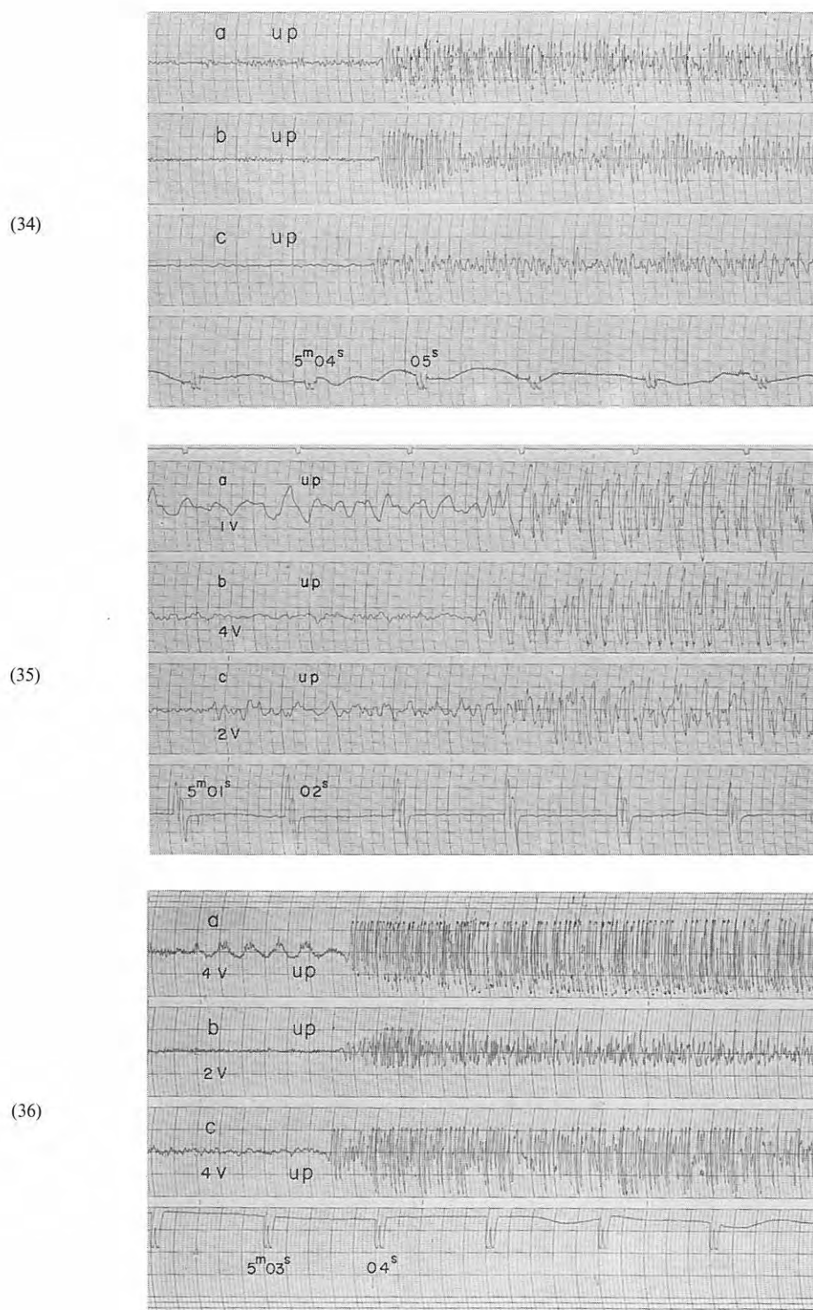
Fig. 5-12 Seismograms obtained (34) at D_2 , (35) at D_3 and (36) at D_4 from the shot A-III
