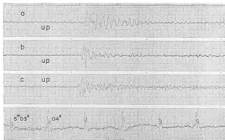
Fig. 5-40 Seismograms obtained (118) at D_5 , (119) at D_6 and (120) at D_7 of profile A from the shot B-IV
