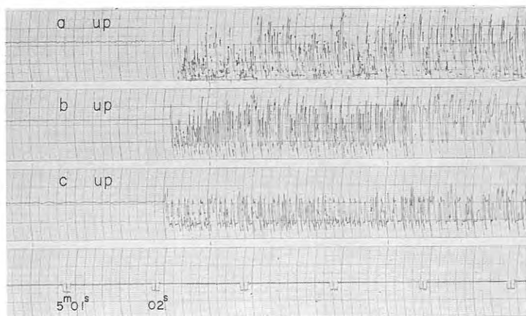
Fig. 5-6 Seismograms obtained (16) at D_{14} from the shot A-I, and (17) at D_1 and (18) at D_2 from the shot A-II
