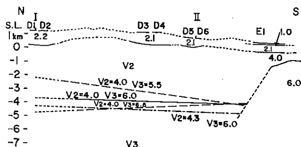
Fig. 17 Various models in the section between B-I and E_1
