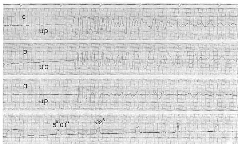
Fig. 5-37 Seismograms obtained (109) at D_{11} , (110) at D_{12} and (111) at D_{13} from the shot A- V_2
