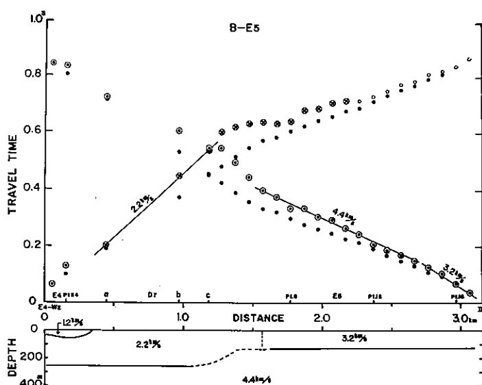
Fig. 14 Travel time curve from the measurement of surface structure at the spread E_5 (above) and the surface structure derived (below). Marks for observed data are the same with those in Fig. 8. Closed circle: T(\text{III}-E_4-W_2)
