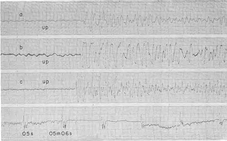
Fig. 5-29 Seismograms obtained (85) at D 5 , (86) at D 6 and (87) at D 7 from the shot A-V 1
