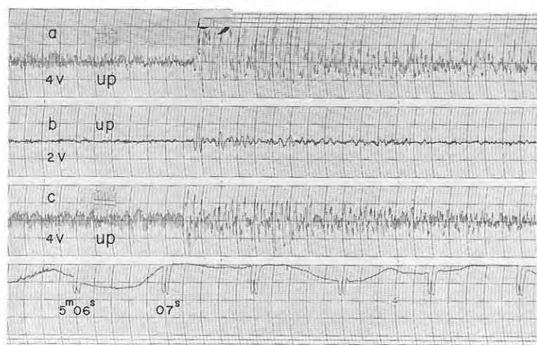
Fig. 5-39 Seismograms obtained (115) at D 2 , (116) at D 3 and (117) at D 4 of profile A from the shot B-IV
