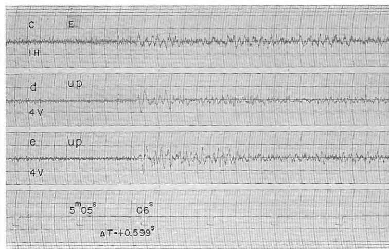
Fig. 5-16 Seismograms obtained (46) at D_{13} , (47), (48) at D_{14} from the shot A-III
