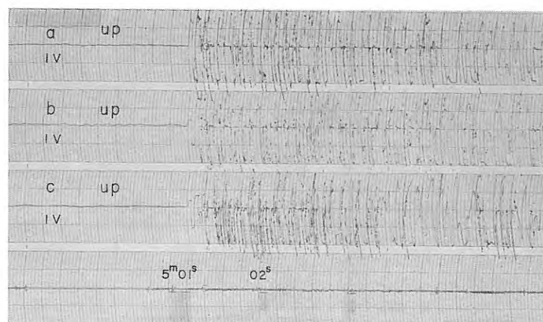
Fig. 5-7 Seismograms obtained (19) at D 3 , (20) at D 4 and (21) at D 5 from the shot A-II
