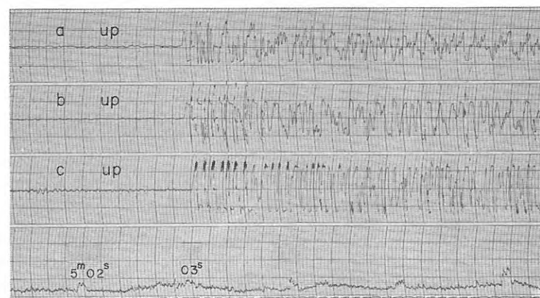
Fig. 5-14 Seismograms obtained (40) at D_8 , (41) at D_8' and (42) at D_9 from the shot A-III
