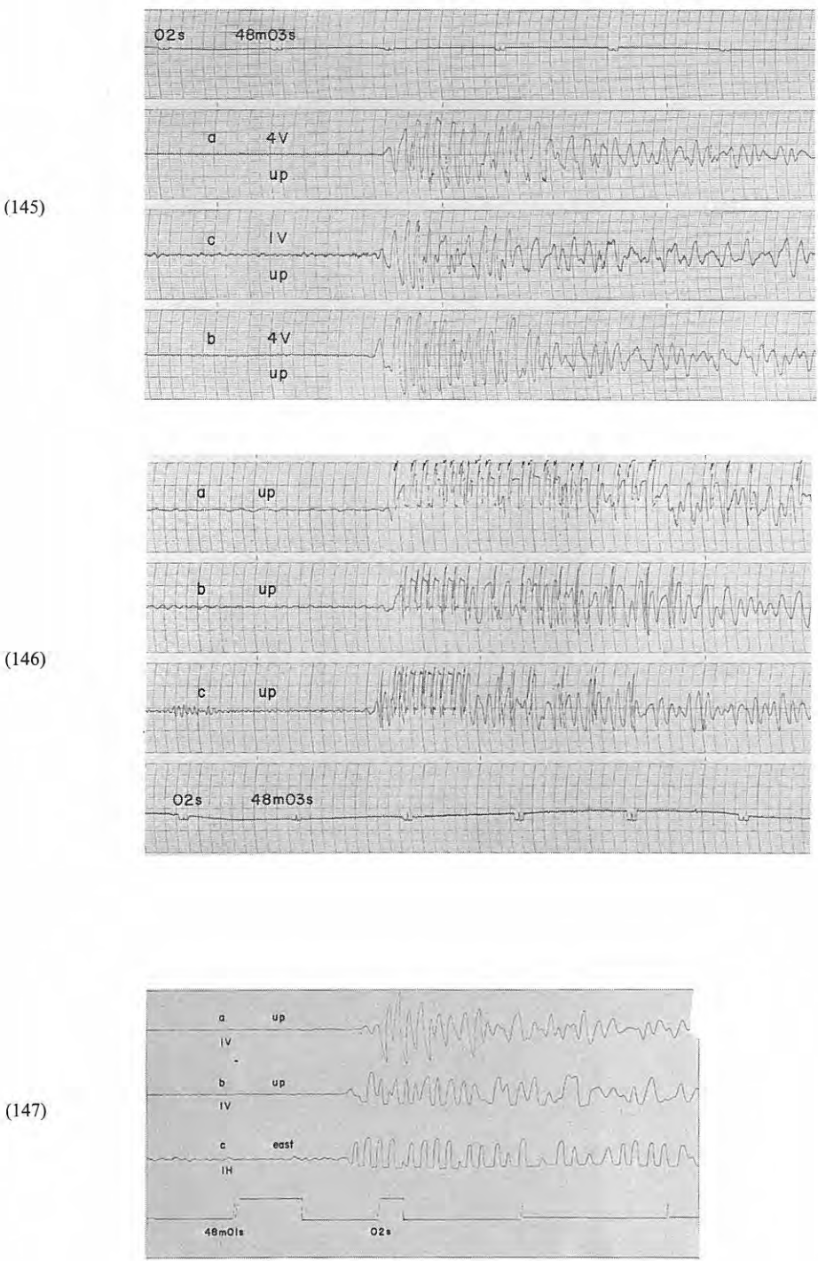
Fig. 5-49 Seismograms obtained (145) at D 1 , (146) at D 2 and (147) at D 3 from the shot B-II
