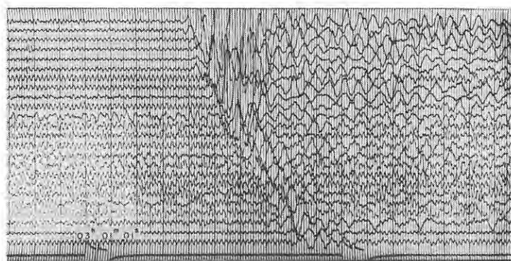
Fig. 6-26 Seismograms obtained (76) at E_5 from the shot E_4-W_2
