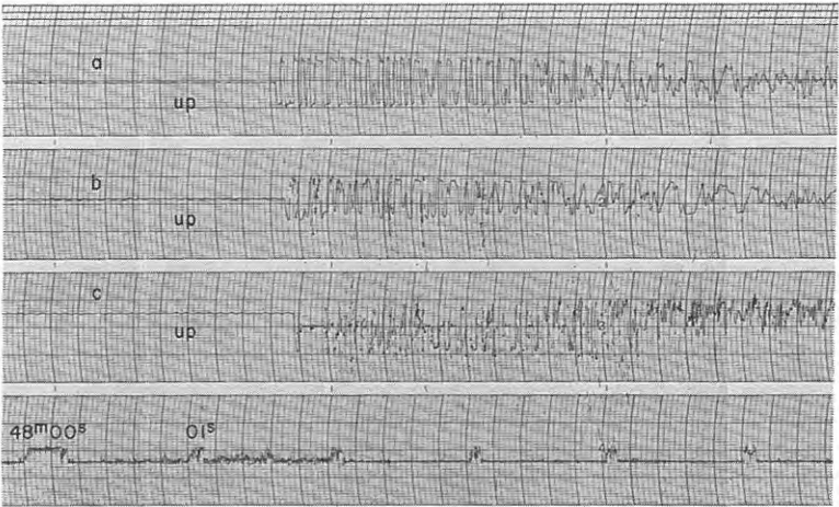
Fig. 5-61 Seismograms obtained (181) at D_8 , (182) at D_9 and (183) at D_{10} from the shot B-III 2
