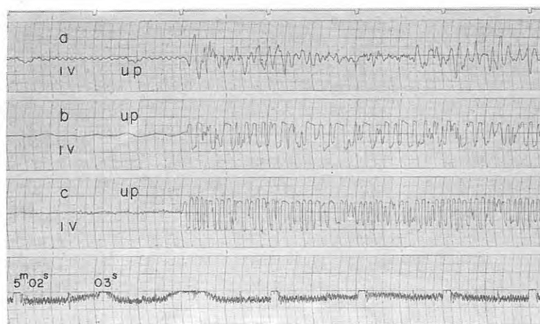
Fig. 5-18 Seismograms obtained (52) at D_4 , (53) at D_5 and (54) at D_6 from the shot A-IV 1
