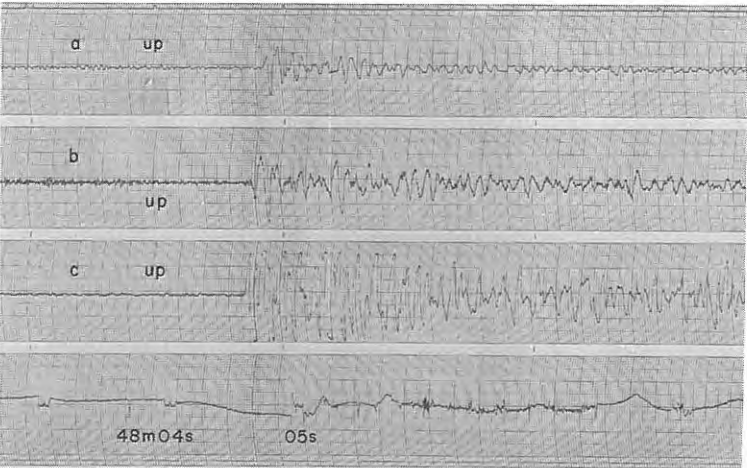
Fig. 5-65 Seismograms obtained (193) at D 5 , (194) at D 6 and (195) at D 7 from the shot B-IV
