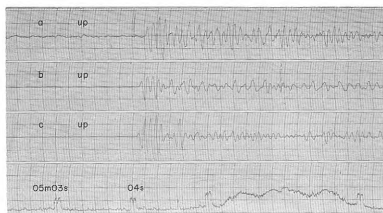
Fig. 5-30 Seismograms obtained (88) at D_8 , (89) at D_8' and (90) at D_9 from the shot A-V 1
