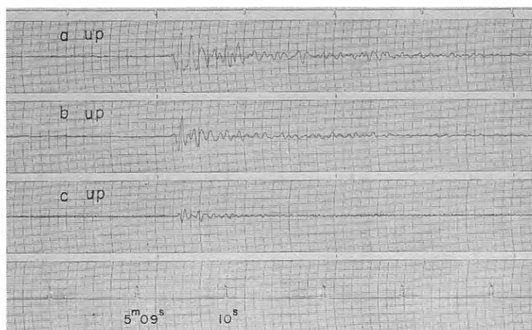
Fig. 5-4 Seismograms obtained (10) at D_9 , (11) at D_{10} and (12) at D_{11} from the shot A-I
