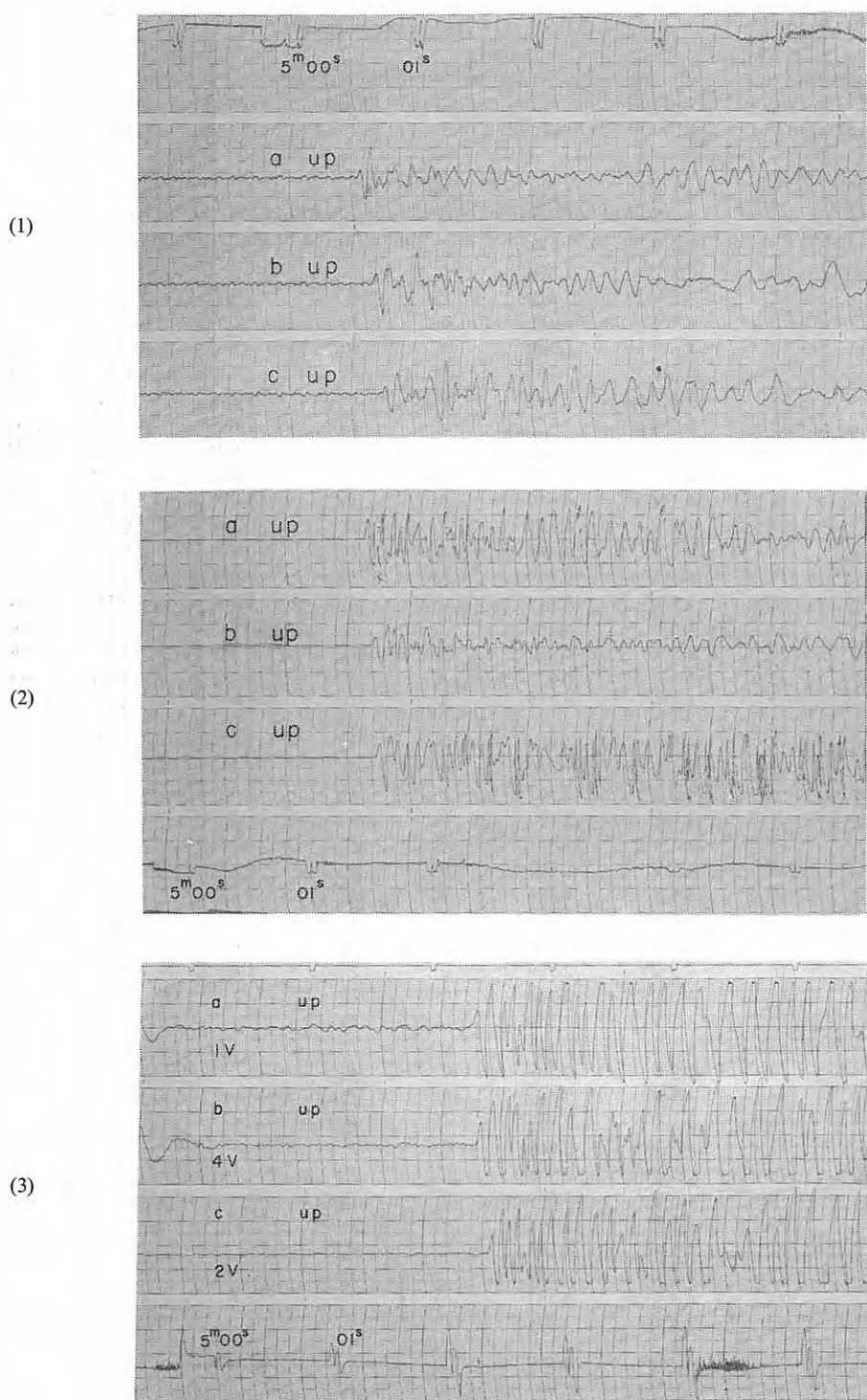
Fig. 5-1 Seismograms obtained (1) at D_1 , (2) at D_2 and (3) at D_3 from the shot A-I
