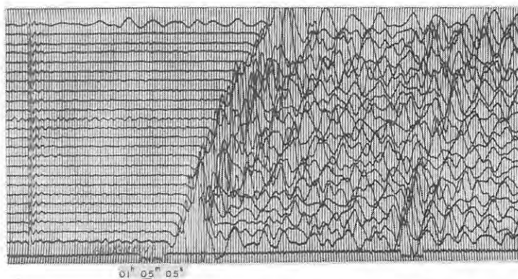
Fig. 6-7 Seismograms obtained (19) at E_4 and (20) at E_5 from the shot A-IV 1 , and (21) at E_1 from the shot A-IV 2
