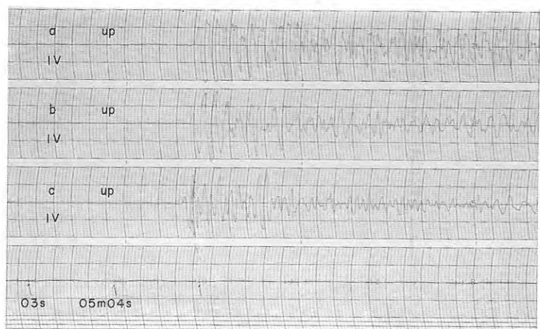
Fig. 5-23 Seismograms obtained (67) at D_3 , (68) at D_4 and (69) at D_5 from the shot A-IV 2
