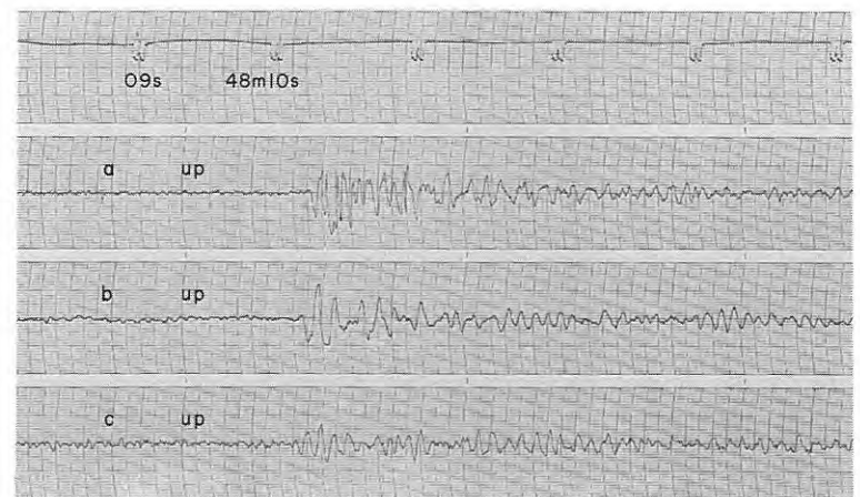
Fig. 5-63 Seismograms obtained (187), (188) at D_{14} from the shot B-III 2 , and (189) at D_1 from the shot B-IV
