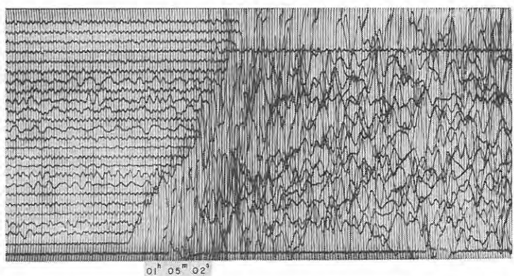
Fig. 6-8 Seismograms obtained (22) at E_2 , (23) at E_3 and (24) at E_4 from the shot A-IV 2
