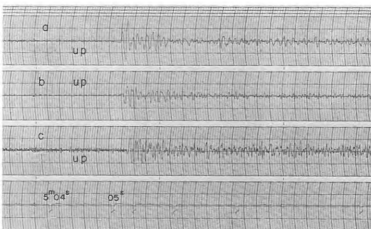
Fig. 5-42 Seismograms obtained (124) at D_{10} , (125) at D_{11} and (126) at D_{12} of profile A from the shot B-IV
