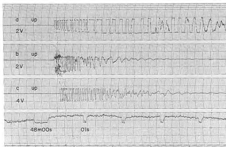
Fig. 5-50 Seismograms obtained (148) at D_4 , (149) at D_5 and (150) at D_6 from the shot B-II
