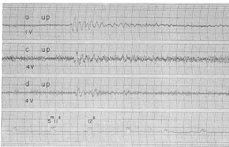
Fig. 5-5 Seismograms obtained (13) at D_{12} , (14) at D_{13} and (15) at D_{14} from the shot A-I
