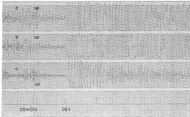
Fig. 5-20 Seismograms obtained (58) at D 9 , (59) at D 10 and (60) at D 11 from the shot A-IV 1
