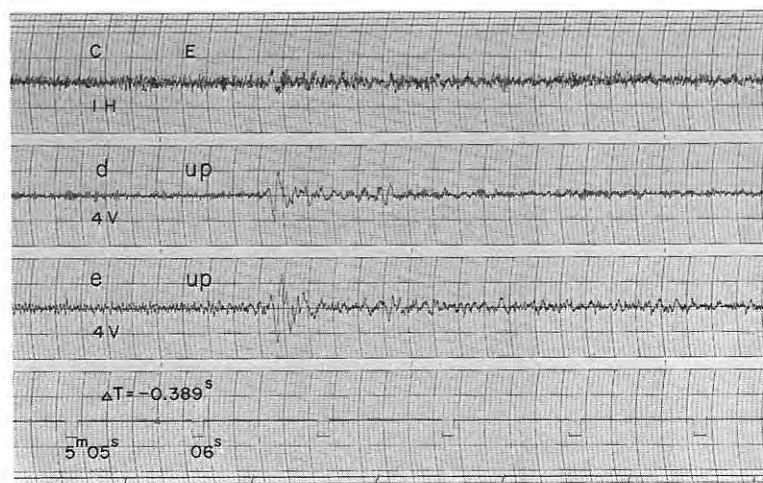
Fig. 5-43 Seismograms obtained (127) at D_{13} , (128), (129) at D_{14} of profile A from the shot B-IV
