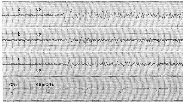
Fig. 5-51 Seismograms obtained (151) at D 7 , (152) at D 8 and (153) at D 9 from the shot B-II
