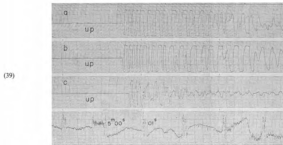
Fig. 5-13 Seismograms obtained (37) at D_5 , (38) at D_6 and (39) at D_7 from the shot A-III
