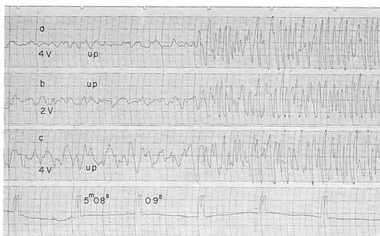
Fig. 5-28 Seismograms obtained (82) at D_2 , (83) at D_3 and (84) at D_4 from the shot A- V_1
