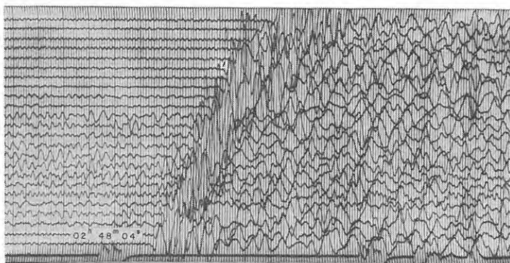
Fig. 6-21 Seismograms obtained (61) at E_3 , (62) at E_4 and (63) at E_5 from the shot B-IV
