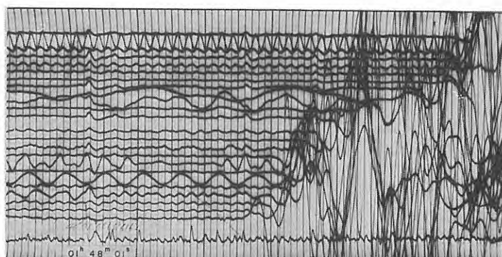
Fig. 6-19 Seismograms obtained (55) at E_2 , (56) at E_3 and (57) at E_4 from the shot B-III 2
