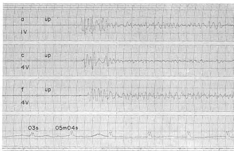
Fig. 5-21 Seismograms obtained (61) at D_{12} , (62) at D_{13} and (63) at D_{14} from the shot A-IV 1
