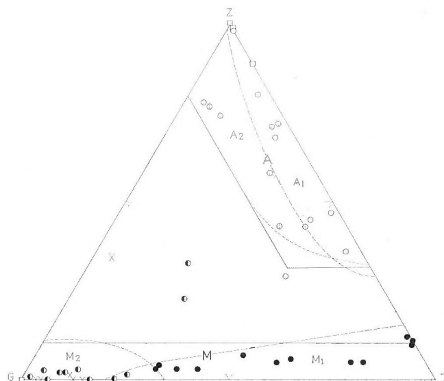
Fig. 24 ZGT diagram of granite, crystalline schist, gneiss, and sediments of the above origin.
