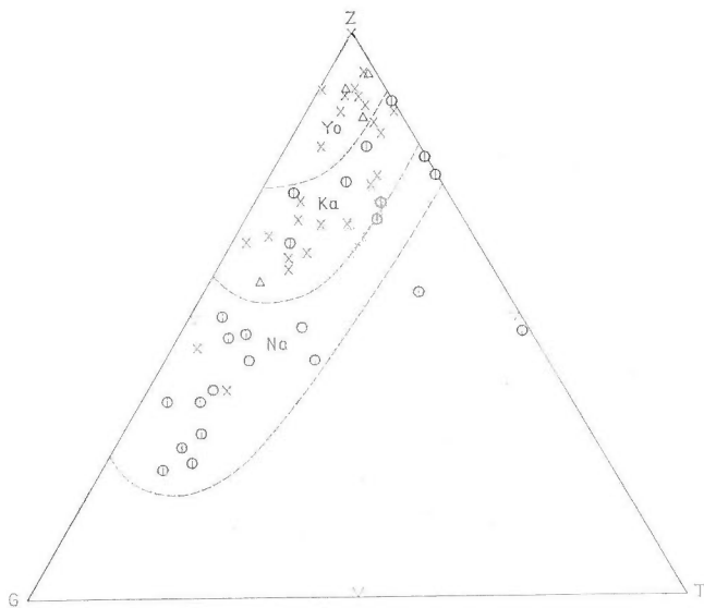
Fig. 11 ZGT diagram of the Ōmura (Nanaura formation) and Manda groups of the Miike coal field. Δ, Yotsuyama formation; x, Kattachi formation; ⊙, Nanaura formation.
